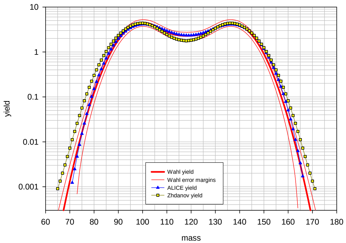
Benchmark B: ^{237}\text{Np} at 28 MeV, pre-neutron emission mass distribution
